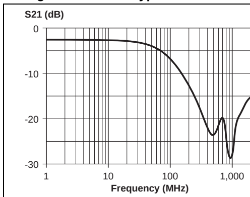
Figure 4. USBUFF typical attenuation
