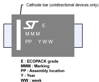
Figure 19. SMA marking
