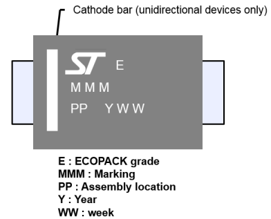
Figure 19. Marking layout
