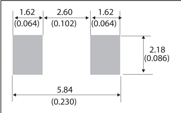
Figure 17. SMB footprint dimensions in mm (inches)
