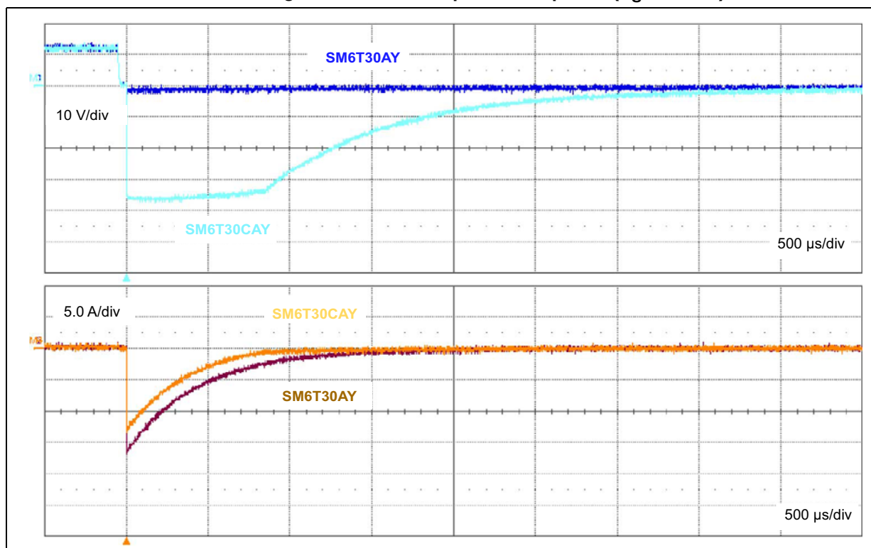
Figure 6. ISO 7637-2 pulse 1 response ( V_S = -150\text{ V} )
