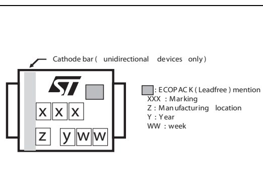
Figure 14. Marking layout (1)
