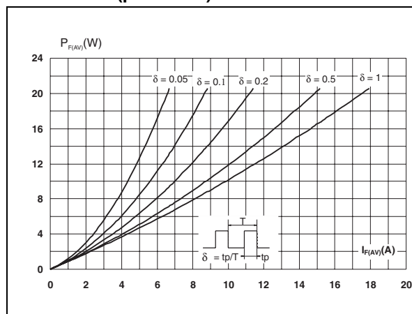
Figure 1. Average forward power dissipation versus average forward current (per diode)
