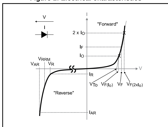
Figure 1: Electrical characteristics
