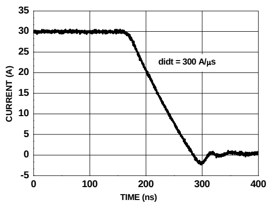
Figure 27. FDMS3660S SyncFET™ body diode reverse recovery characteristic
