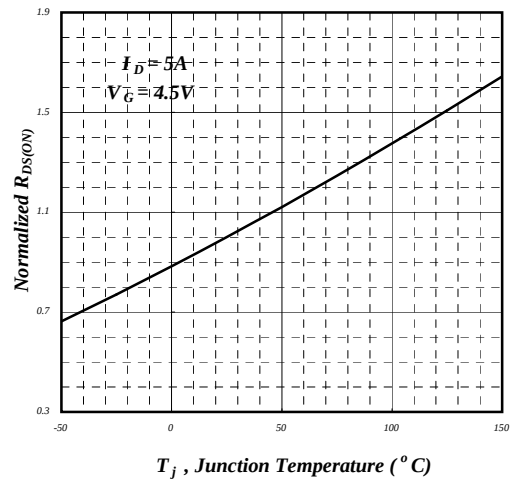
Fig 4. Normalized On-Resistance
