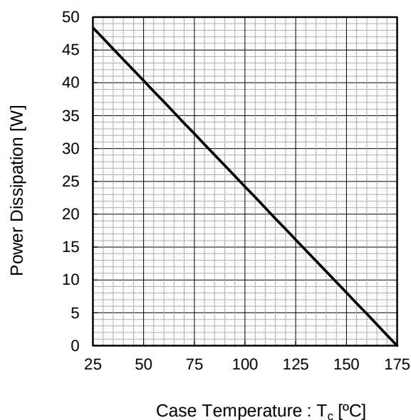
Fig.6 Power Dissipation
