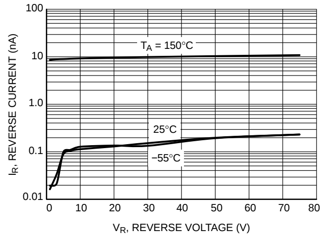
Figure 4. Leakage Current
