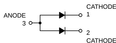
SC-70 CASE 419 STYLE 4
