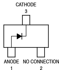
SC-70 (SOT-323) CASE 419 STYLE 2
