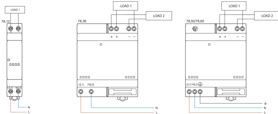
Dual connection
