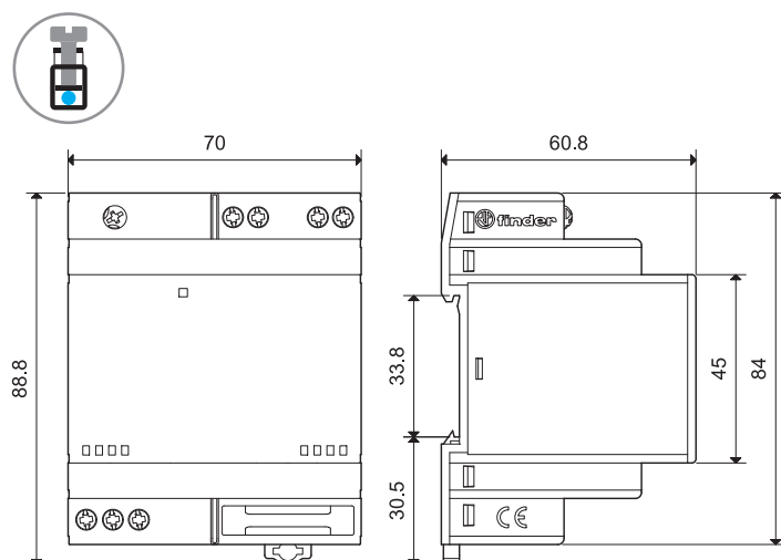
78.50 / 78.60 Screw terminal
