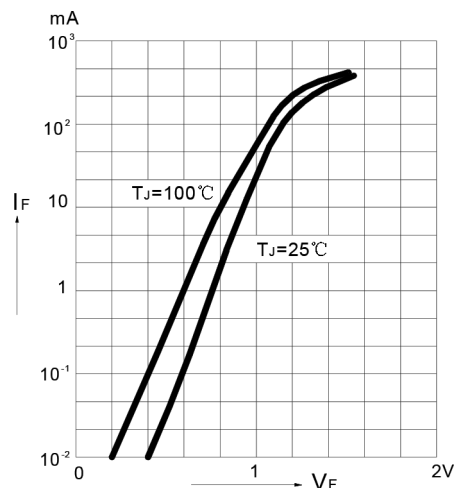
FIG.2 – FORWARD CHARACTERISTICS
