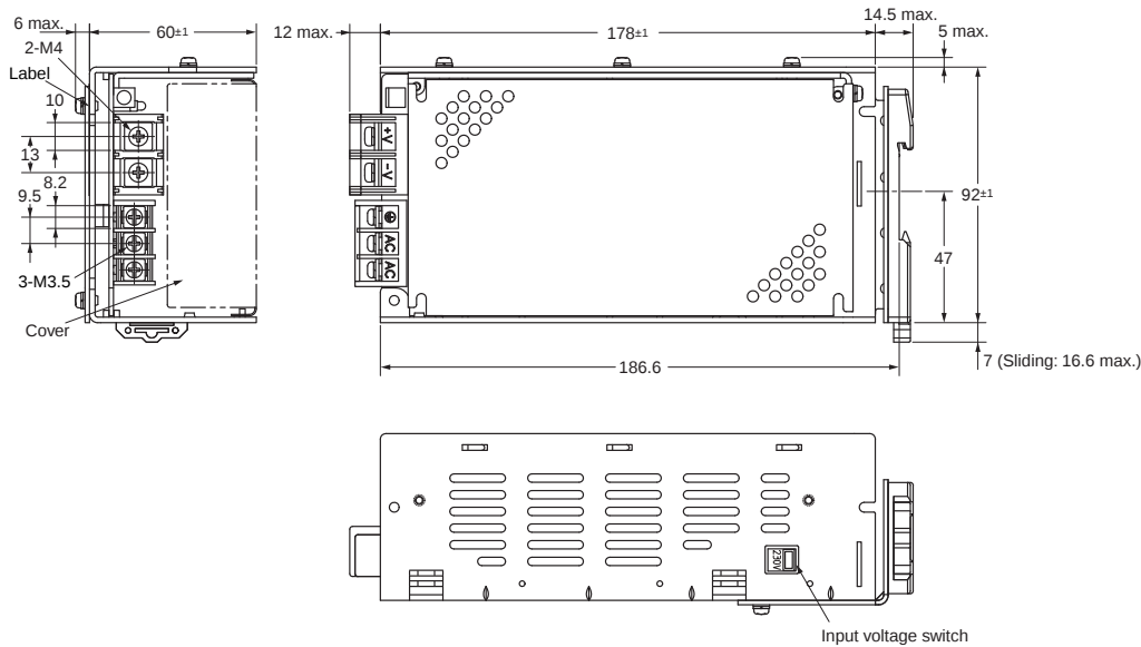
S8JX-G15005D (150 W) S8JX-G15005CD (150 W)
