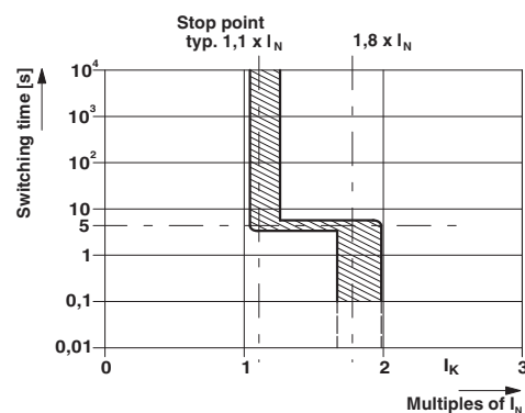
Trigger characteristic
