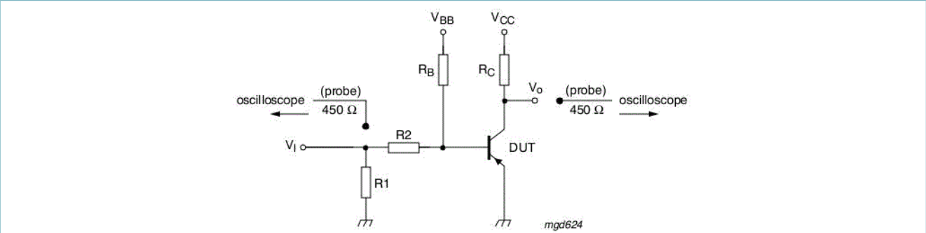
Fig. 29. TR2 (PNP): Test circuit for switching times
