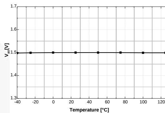
Figure 20. V_{RT} vs. Temperature
