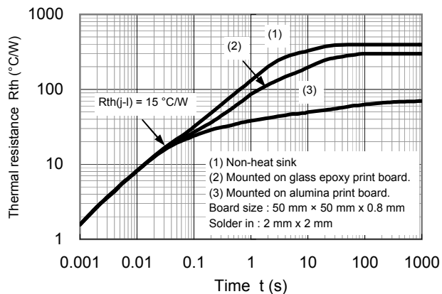
Rth - t
