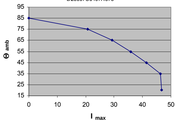
Max. allowable ambient Temp. at specific current (rms) B25667C3497A375
