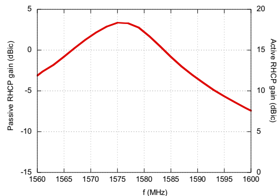
Active/Passive gain vs. frequency
