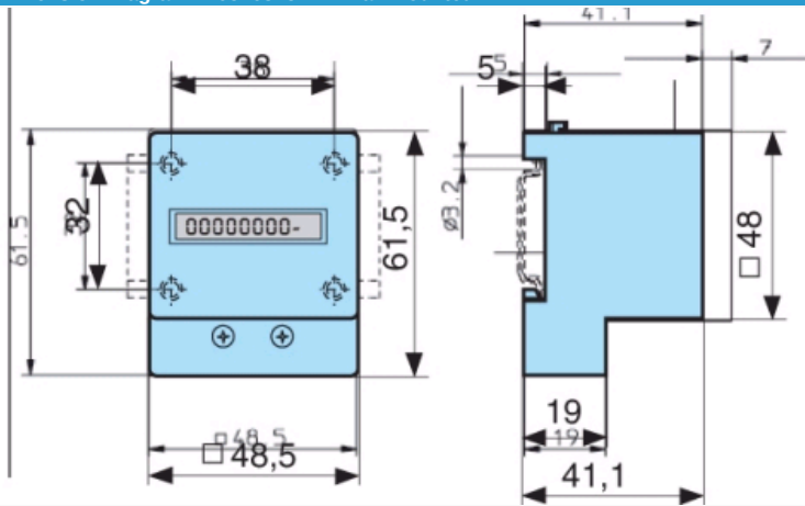
Dimension Diagram : 26546845 - DIN rail mounted
