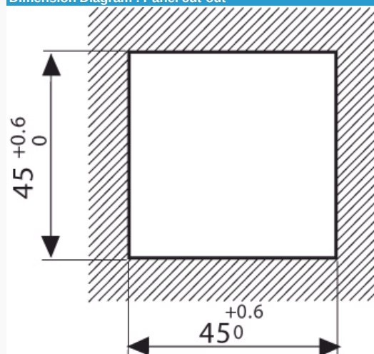
Dimension Diagram : Panel cut-out
