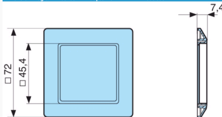
Dimension Diagram : 26546842 - Adaptor for 72 x 72 mm cut-out
