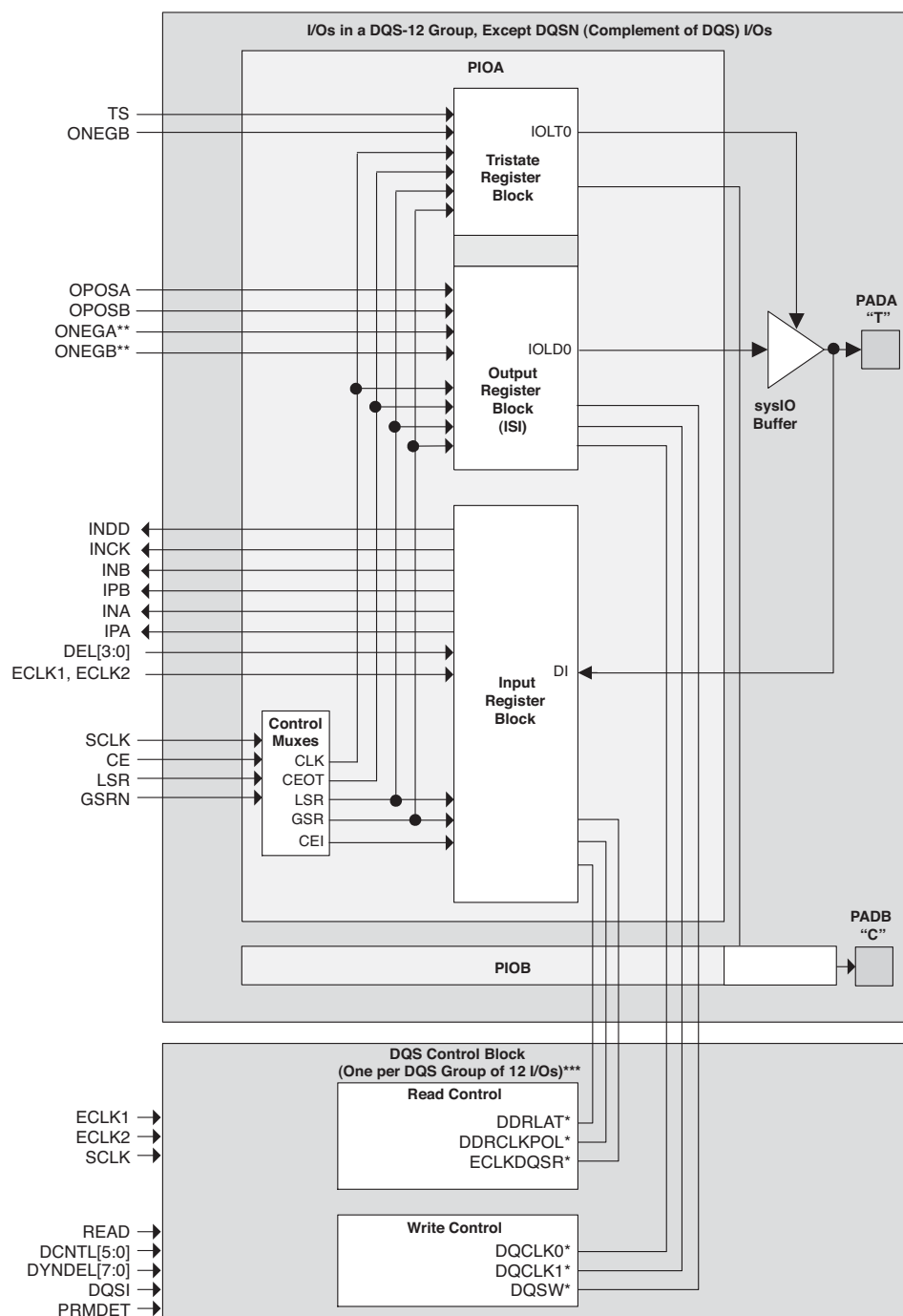
Figure 2-32. PIC Diagram
