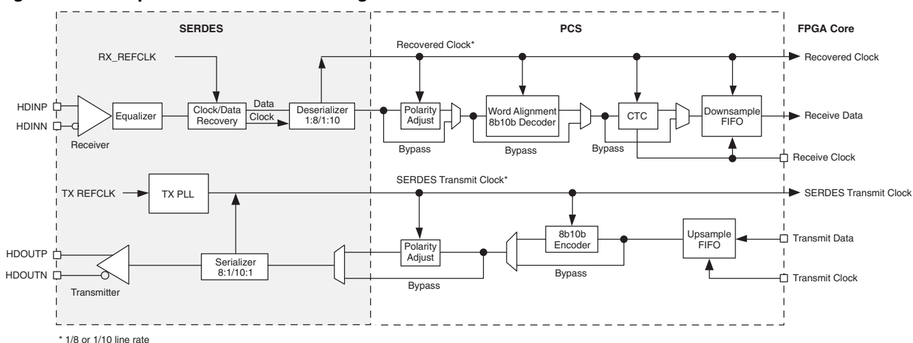
Figure 2-41. Simplified Channel Block Diagram for SERDES/PCS Block
