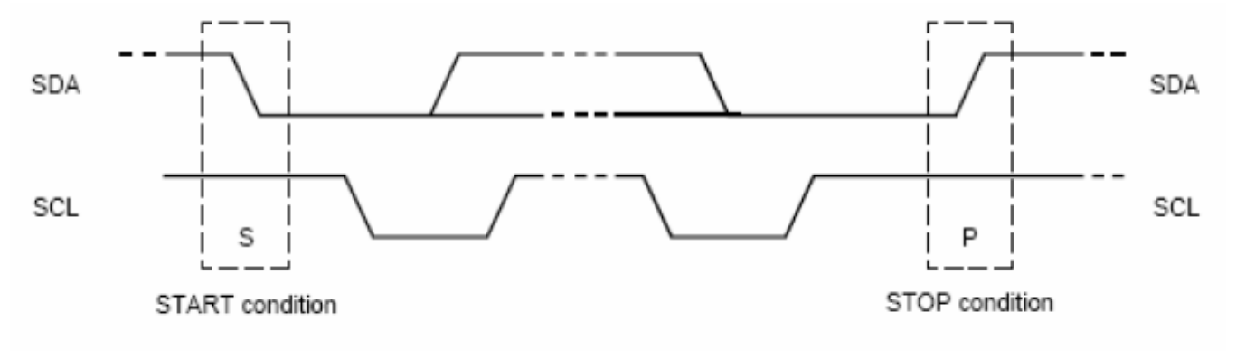
Figure -5: START and STOP conditions
