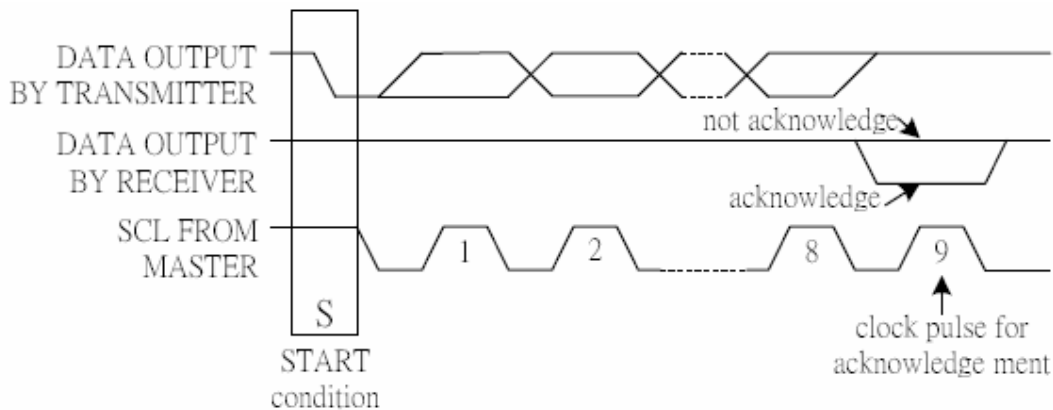
Fig 4 Acknowledgement on the 2-line Interface
