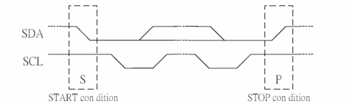
Fig 2 Definition of START and STOP conditions
