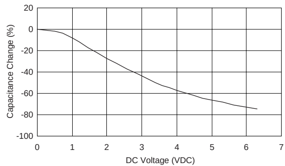
[DC Voltage Characteristics]
