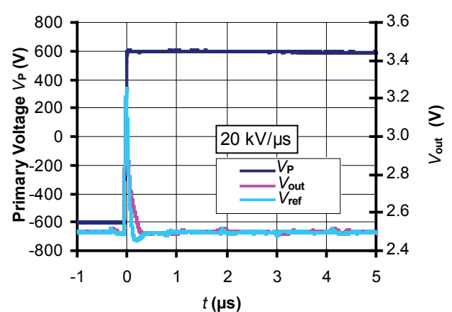
Figure 22: Step response
