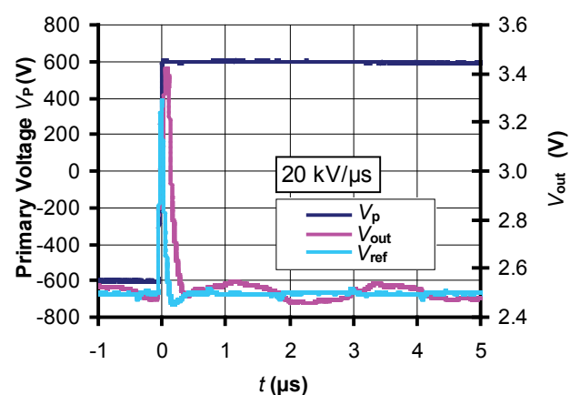
Figure 6: dv/dt
