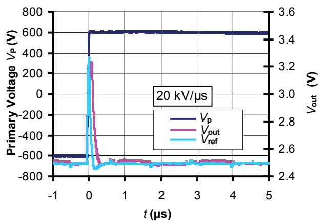
Figure 12: dv/dt
