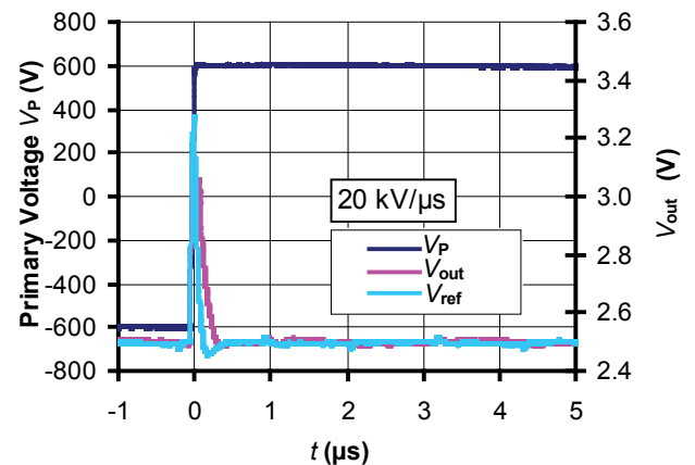
Figure 18: dv/dt
