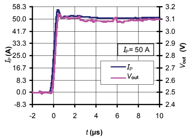
Figure 22: Step response
