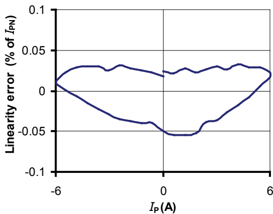
Figure 1: Linearity error
