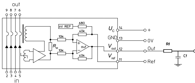
Figure 31: Test connection
