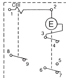
Schematic Diagram "REVERSE START"
