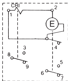
Schematic Diagram "STANDARD START"
