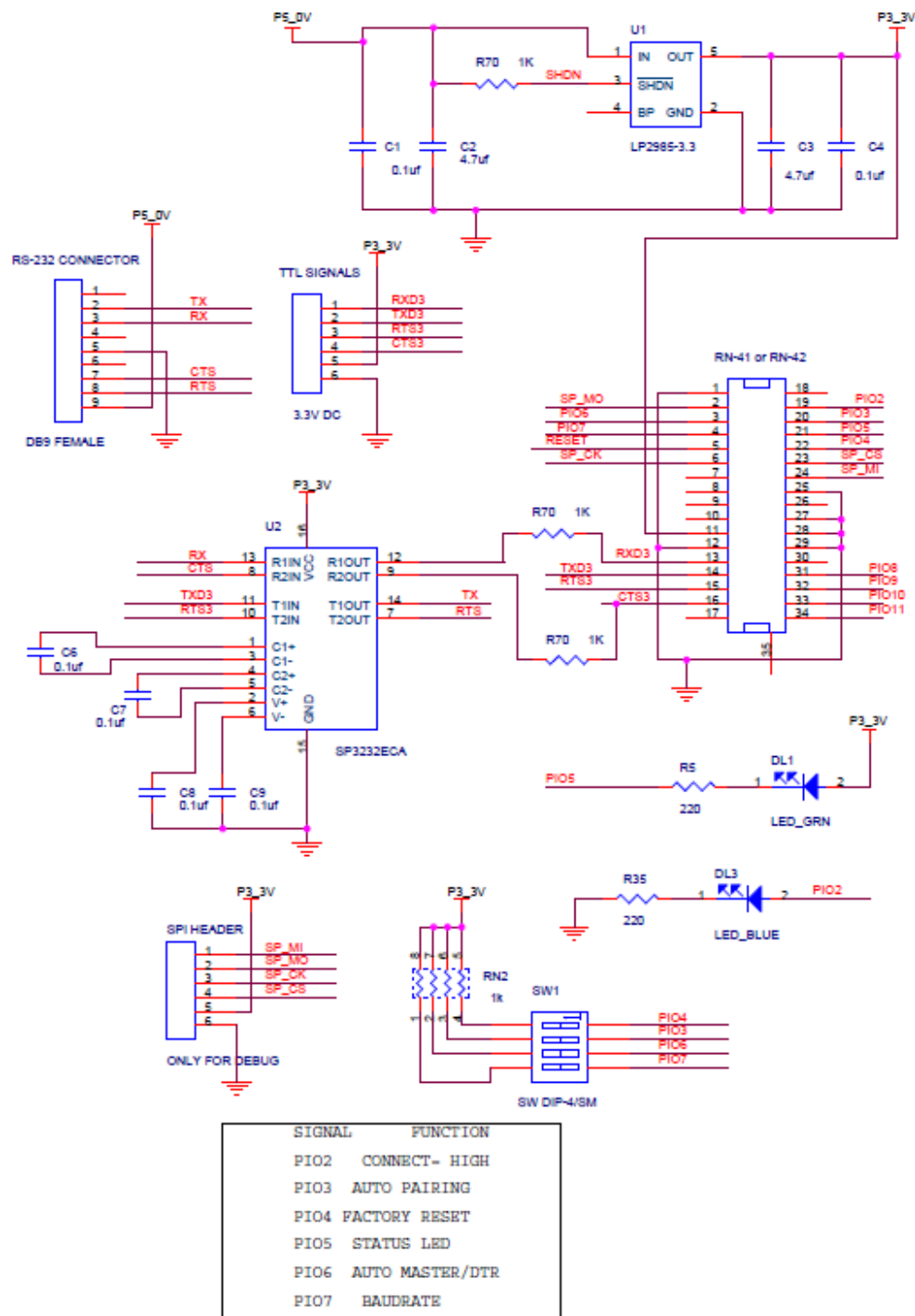
Figure 4. Application Schematic
