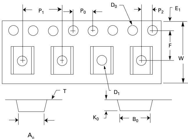
Tape Specifications
