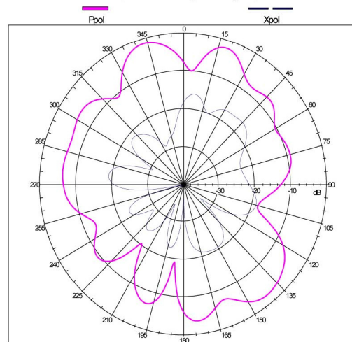
Far-field Pattern @Phi=90 deg(E-Theta Plane-Cut) Gain=-0.58 dBi; Co-Pol Efficiency: 29.35% @Freq: 0.86000 GHz
