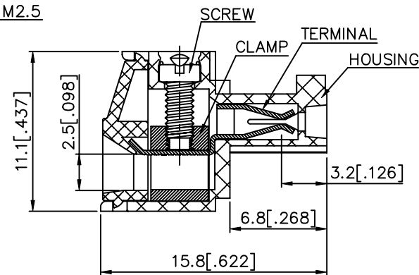
SECTION P-P
