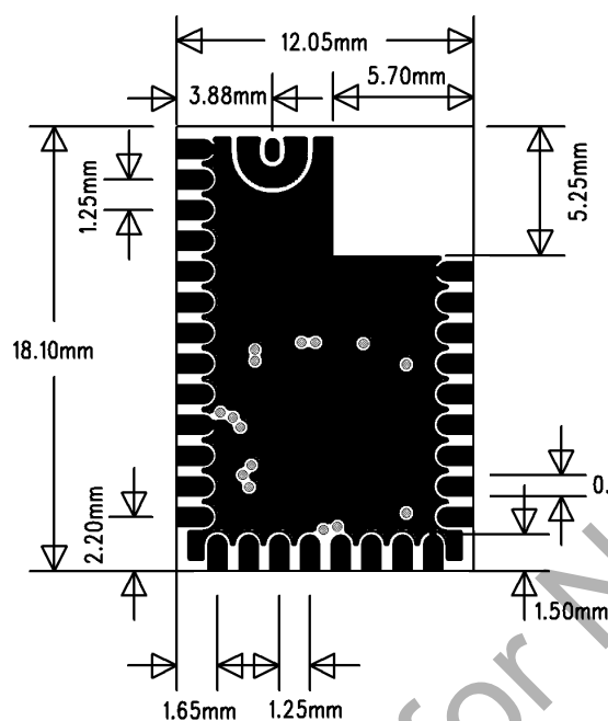
Figure 8: Physical dimensions and pinout (top view)
