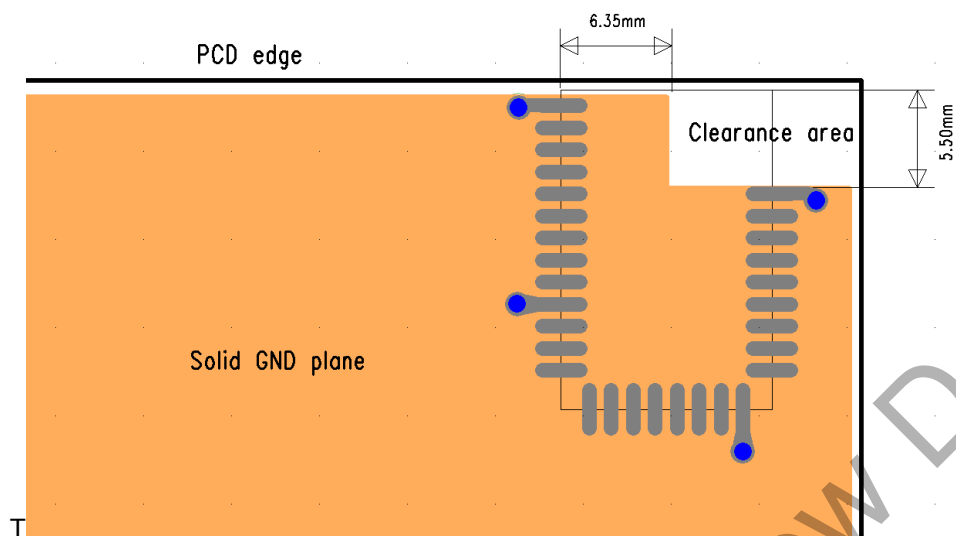
Figure 17: Recommended layout for BLE112-A
