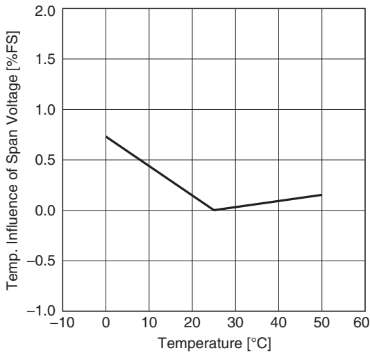
Temperature Influence of Span Voltage
