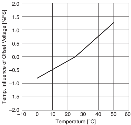
Temperature Influence of Offset Voltage
