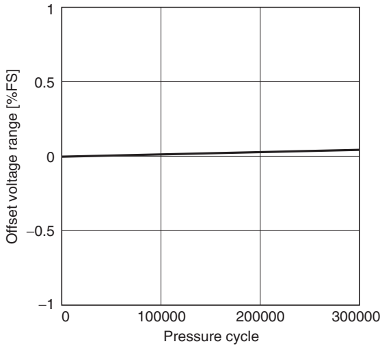
Pressure Cycle Range ( 0 to 40 kPa)
