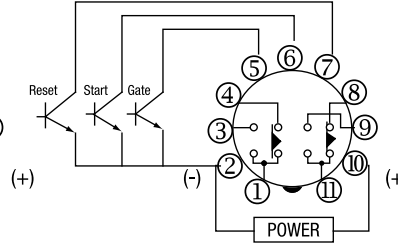
(Transistor Input)
