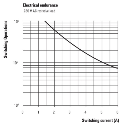
230 V AC resistive load
