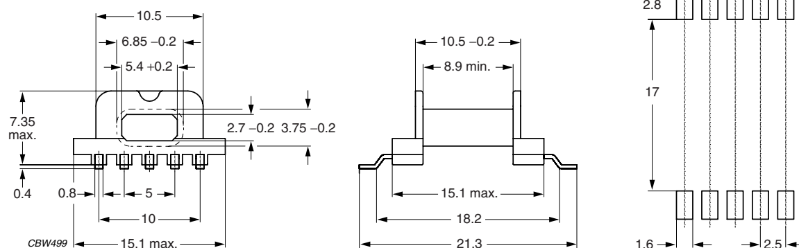
Fig.4 EFD15/8/5 coil former (SMD); 10-solder pads.
