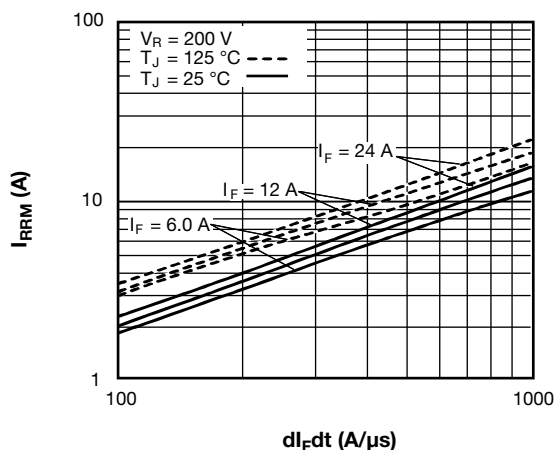
Fig. 15 - Typical Recovery Current vs. dI_F/dt
