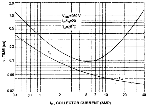
TURN-ON TIME
