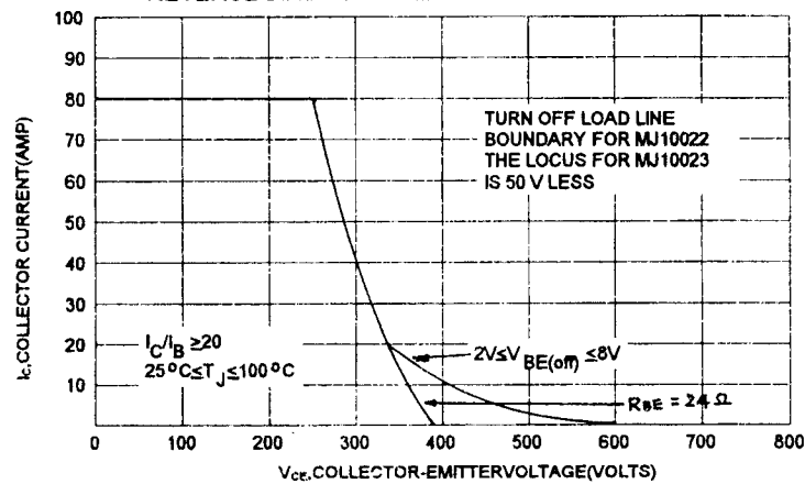
REVERSE BIAS SWITCHING SAFE OPERATING AREA
