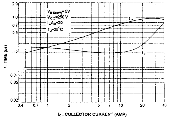
TURN-OFF TIME
