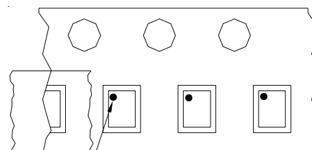
Pin 1 Location
