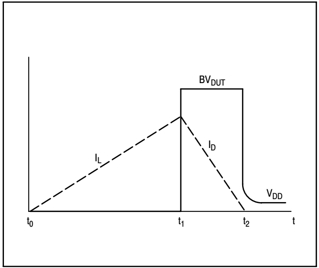
Figure 7. Current-Voltage Waveforms
