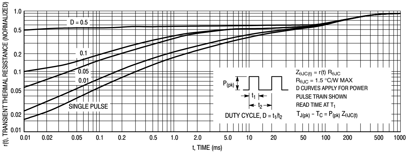
Figure 6. Thermal Response
