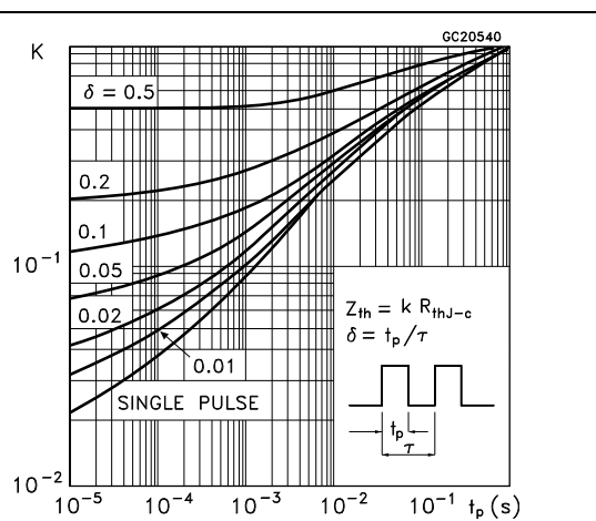
Figure 5. Thermal impedance for TO-220 and D 2 PAK
