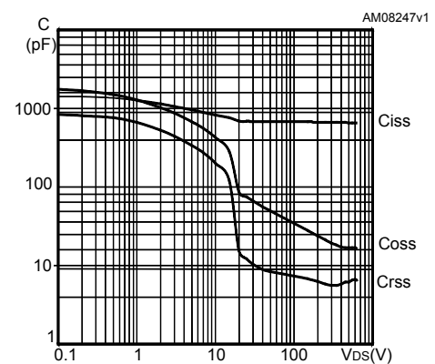
Figure 12. Capacitance variations
