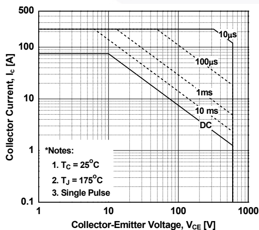
Figure 17. SOA Characteristics
