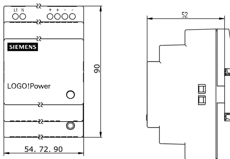
Figure 1-4 Dimension drawing
