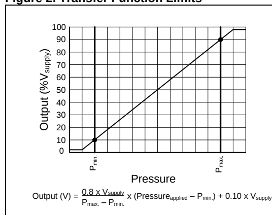
Figure 2. Transfer Function Limits
