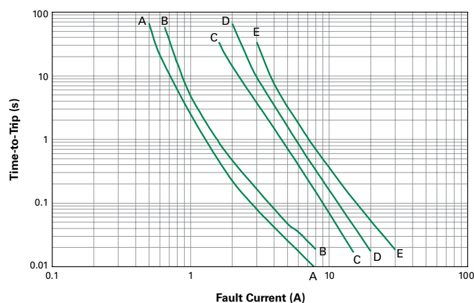
Typical Time-to-Trip Curves at 20°C
