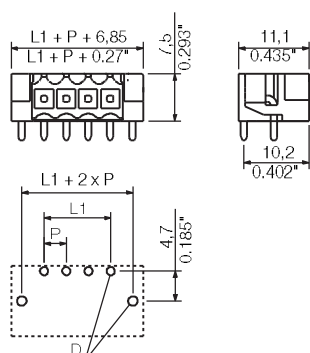
Dimensioned drawing
